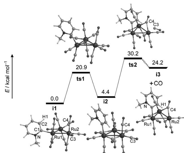
Figure 2. DFT-optimized structures and relative energy profile of the stationary points involved in the transformation of [\text{Ru}_3(\text{CO})_{11}\text{L}] ( \text{L} = N\text{-methylpyrid-2-ylidene} ; i1 ) into i3 + CO.
