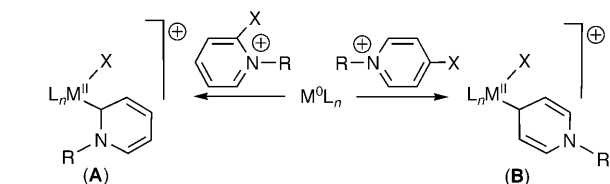
Scheme 1. Syntheses of complexes containing “normal” ( A ) and “remote” ( B ) pyridylidene ligands derived from halopyridinium cations.
